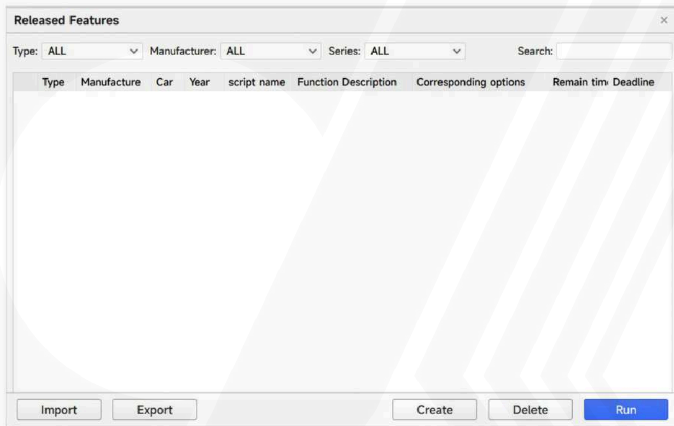
Fig1-2Released Features Interface
