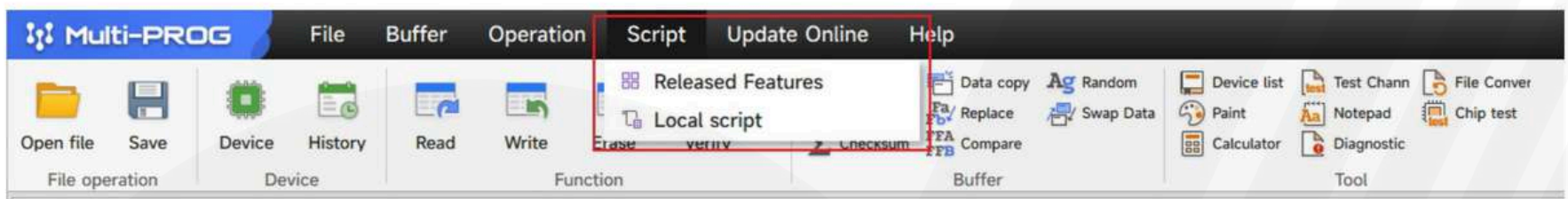
Fig1-1 Script menu
